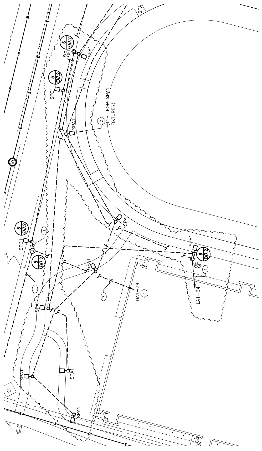
PARTIAL SITE PLAN - BUILDING - LIGHTING SCALE: 1"=30'-0"
