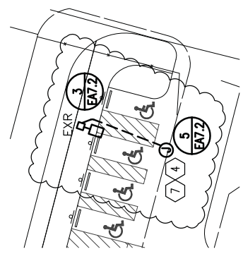
SITE PLAN -- NORTH HALL PARKING -- LIGHTING SCALE: 1"=30'-0"
