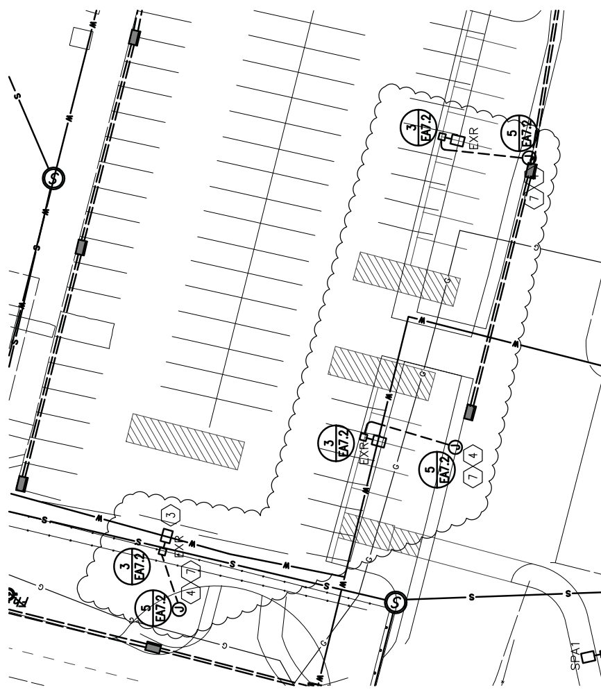
SITE PLAN -- NORTH HALL PARKING -- LIGHTING SCALE: 1"=30'-0"
